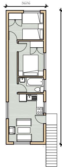
First Floor
